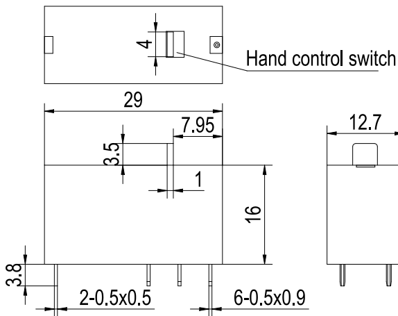
1C2 Outline Dimensions (Double coils latching)
