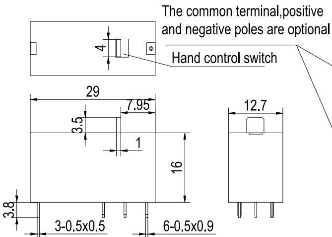
1C2 Outline Dimensions (Double coils latching)
