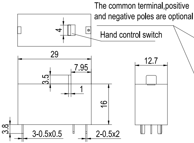
1C2 Outline Dimensions (Single coil latching)
