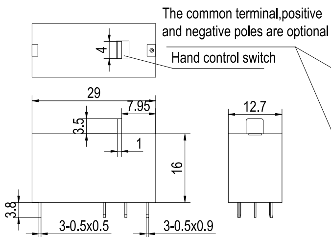
1C5 Outline Dimensions (Double coils latching)
