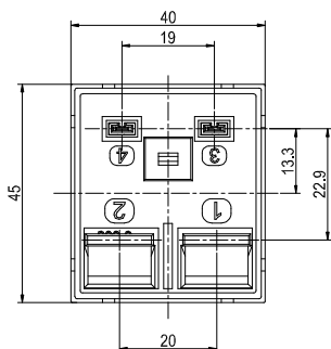
Outline Dimensions
