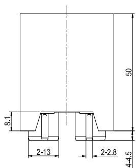
Outline Dimensions
